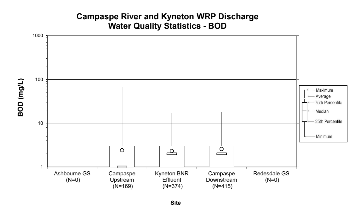
Figure 51 BOD statistics (2015-2021) Kyneton BNR discharge and the Campaspe River
