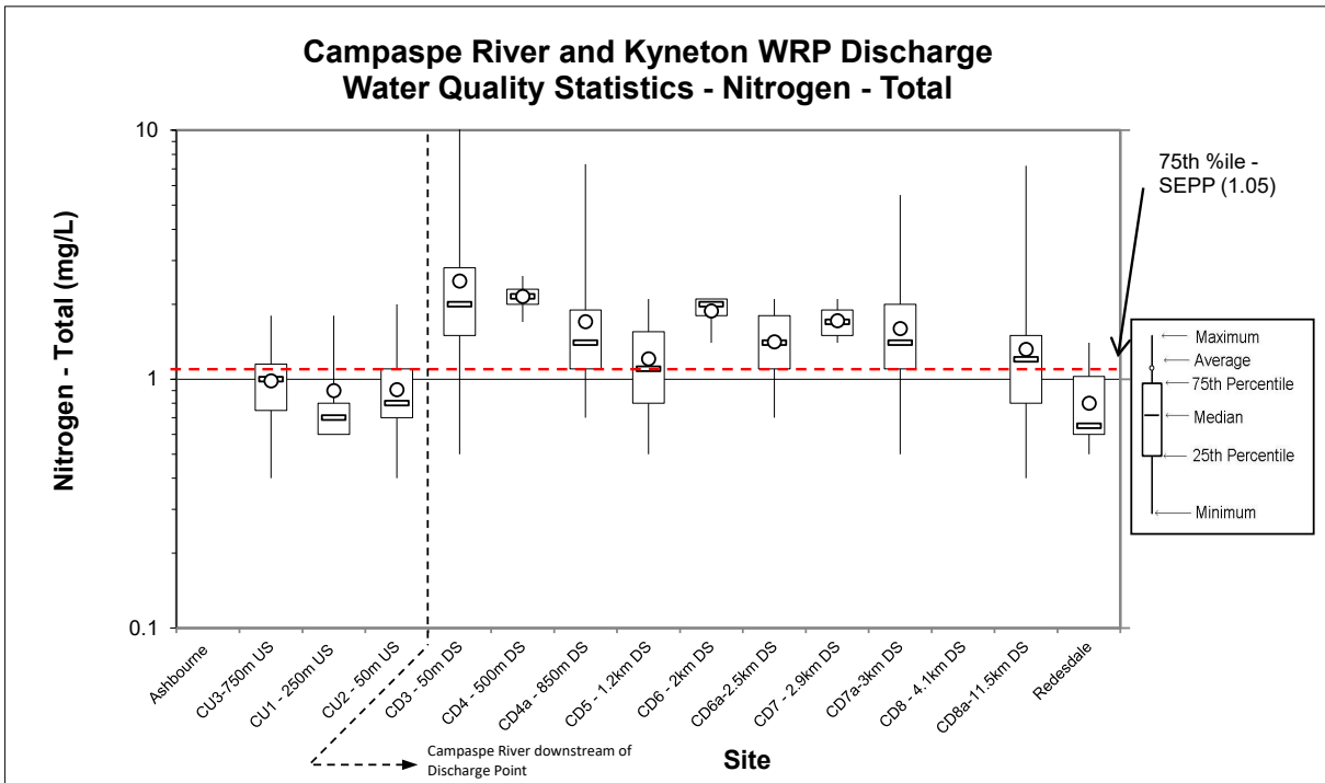
Figure 41 Statistics of total nitrogen data (on discharge days only – July 2020 – December 2021) showing changes in concentration with distance downstream
