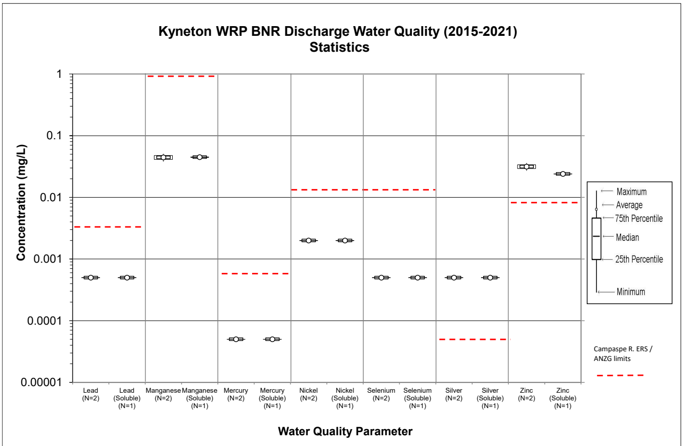
Figure 29 Statistics of metals (lead to zinc) data for the Kyneton BNR discharge (data from 2015-2021)
