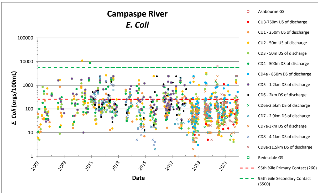
Figure 55 E. coli in Campaspe River upstream and downstream of the discharge point (all data 2007 – 2021)
