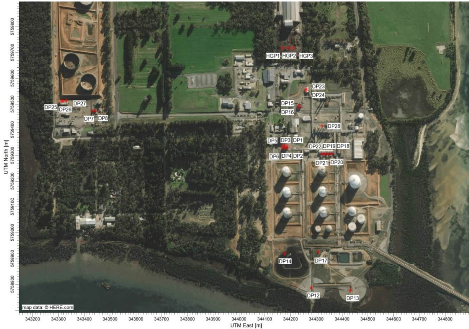
Figure 8 Location of are discharge points at LIP and the project (HGP)
