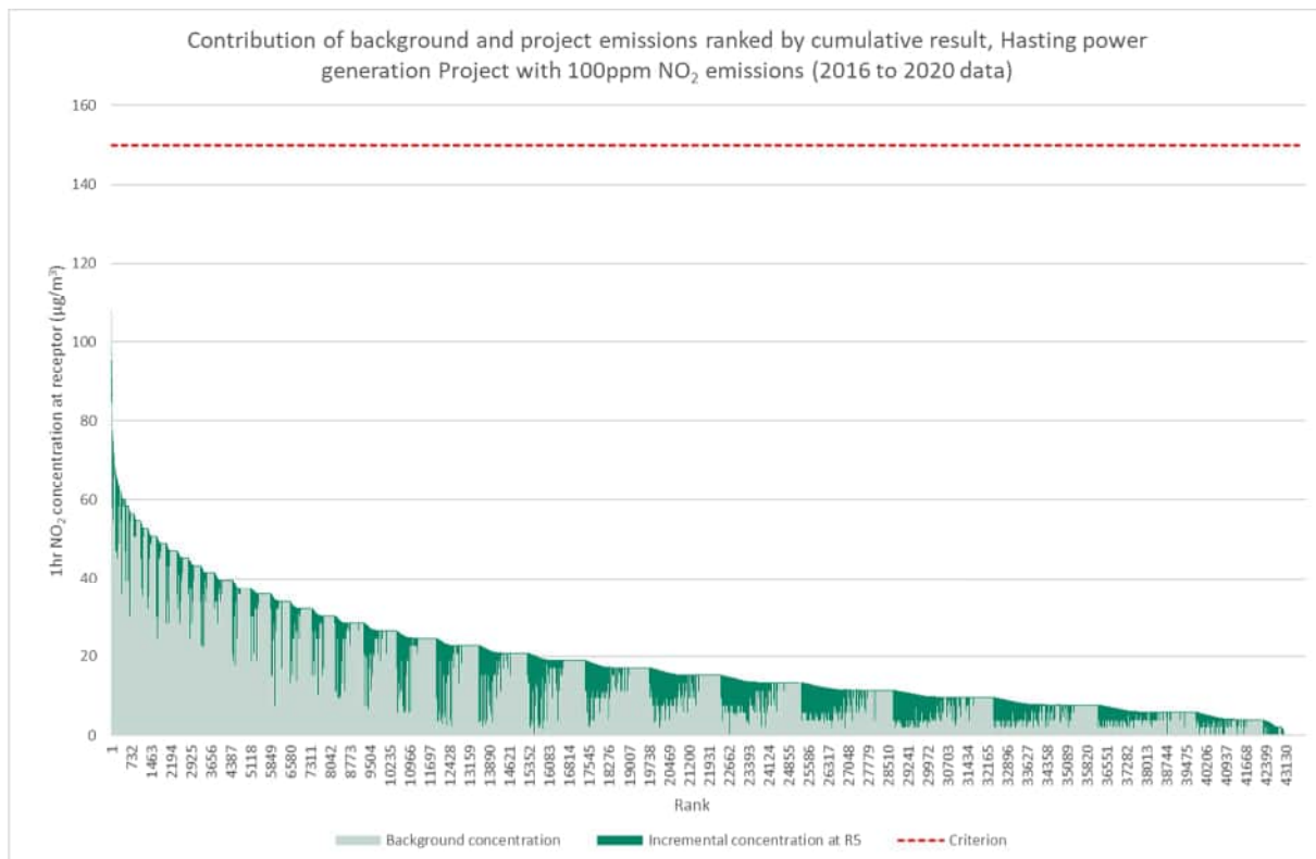
Figure 35 Ranked cumulative NO 2 concentrations at Receptor 5, Hasting power generation Project (with 100ppm NO 2 emissions), 2016 to 2020
