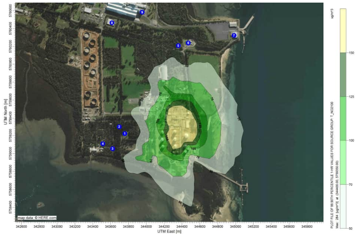
Figure 13 NO 2 results, LIP and Hasting power generation Project with 100ppm NO 2 emissions, 1-hr average 99.9 th percentile, no background, 2016 MET ( \mu\text{g}/\text{m}^3 )
