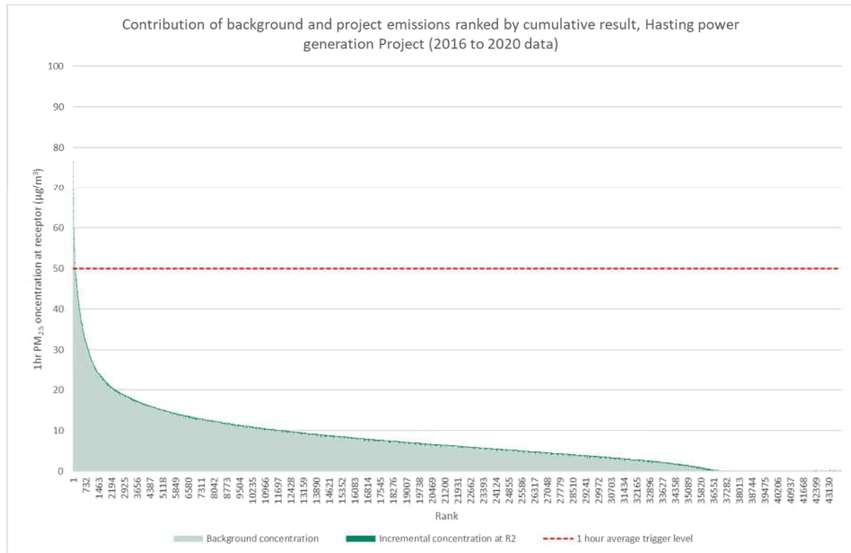
Figure 42 Ranked cumulative PM 2.5 concentrations at Receptor 2, Hasting power generation Project, 2016 to 2020
