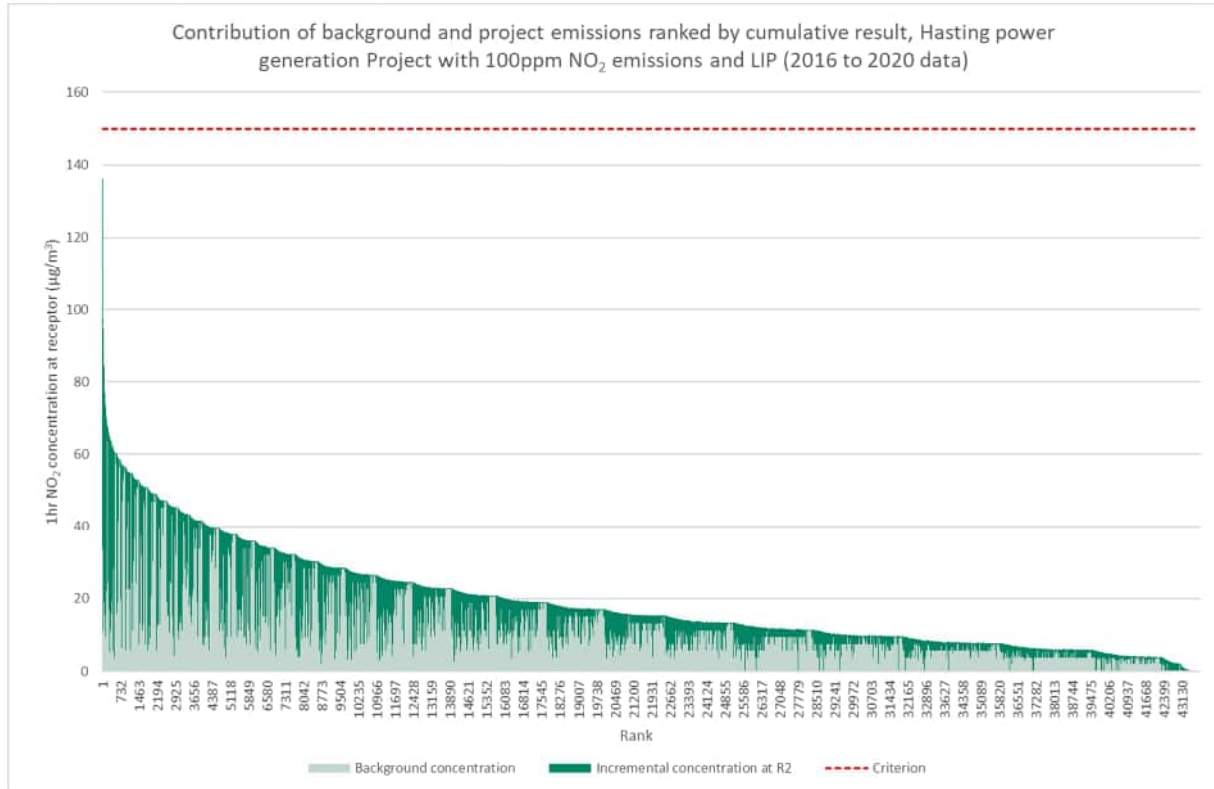
Figure 36 Ranked cumulative NO 2 concentrations at Receptor 2, Hasting power generation Project (with 100ppm NO 2 emissions) and LIP, 2016 to 2020
