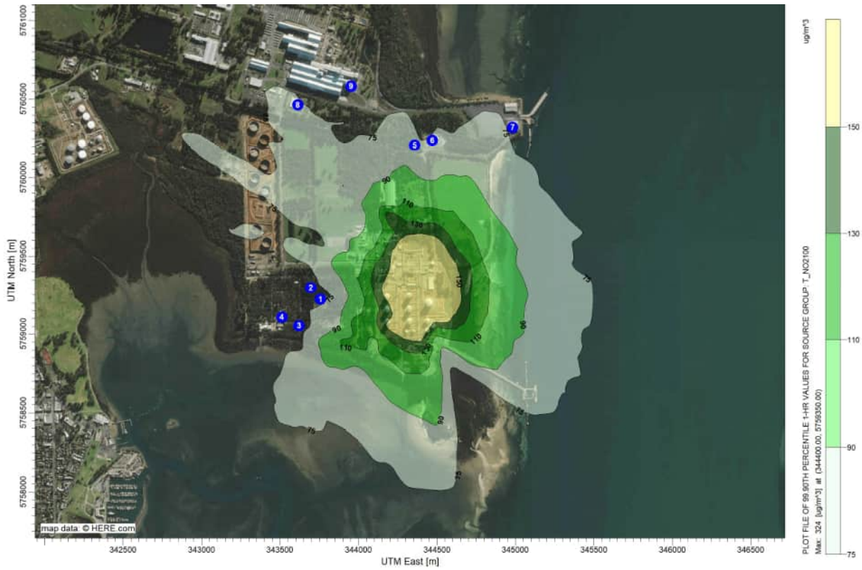
Figure 14 NO 2 results, LIP and Hasting power generation Project with 100ppm NO 2 emissions, 1-hr average 99.9 th percentile, including 39.5 \mu\text{g}/\text{m}^3 background, 2016 MET ( \mu\text{g}/\text{m}^3 )
