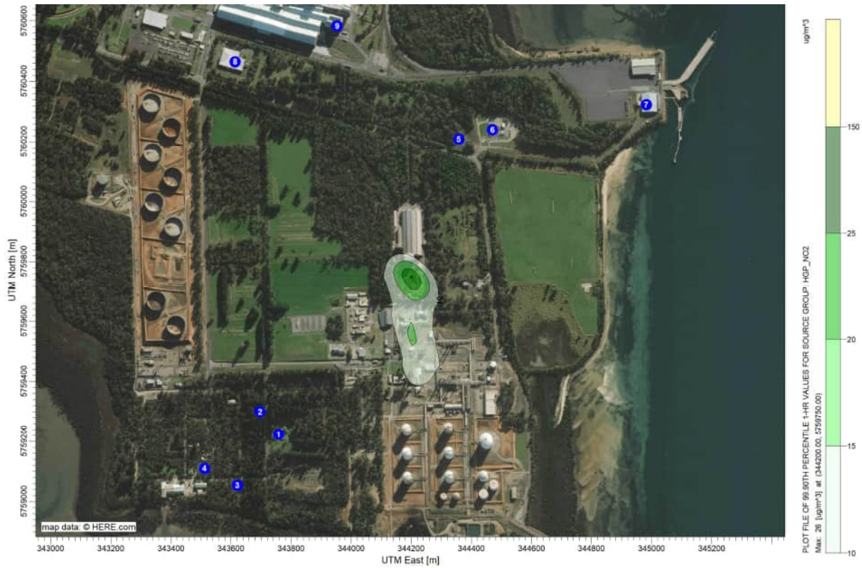
Figure 10 NO 2 results, Hasting power generation Project with 25ppm emissions, 1-hr average 99.9 th percentile, no background, 2016 MET (µg/m 3 )
