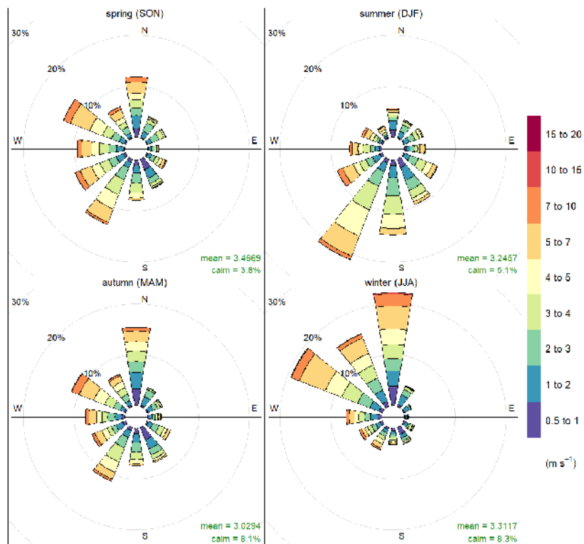
Figure 31 Seasonal wind roses comparison – BoM Cerberus (top) and AERMET (bottom)
