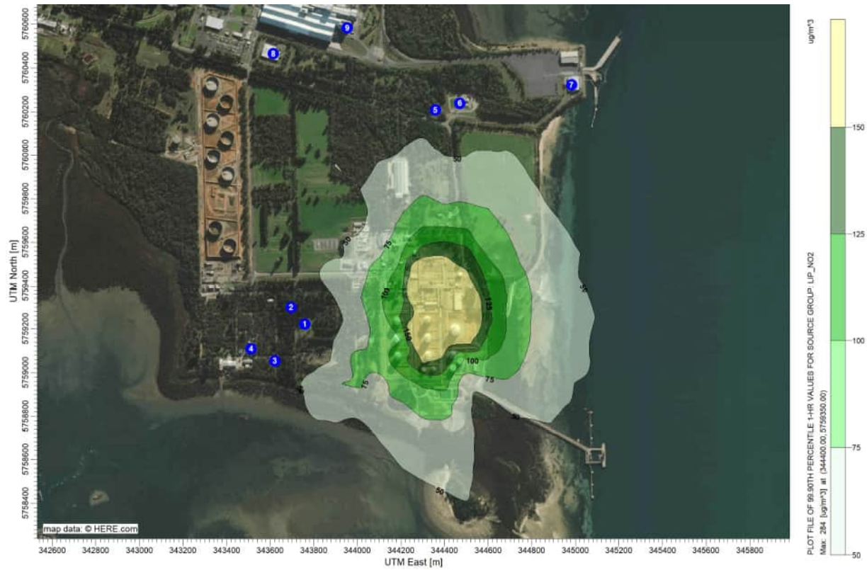
Figure 12 NO 2 results, LIP emissions, 1-hr average 99.9 th percentile, no background, 2016 MET ( \mu\text{g}/\text{m}^3 )
