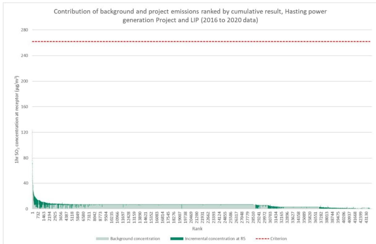
Figure 39 Ranked cumulative SO 2 concentrations at Receptor 5, Hasting power generation Project and LIP, 2016 to 2020
