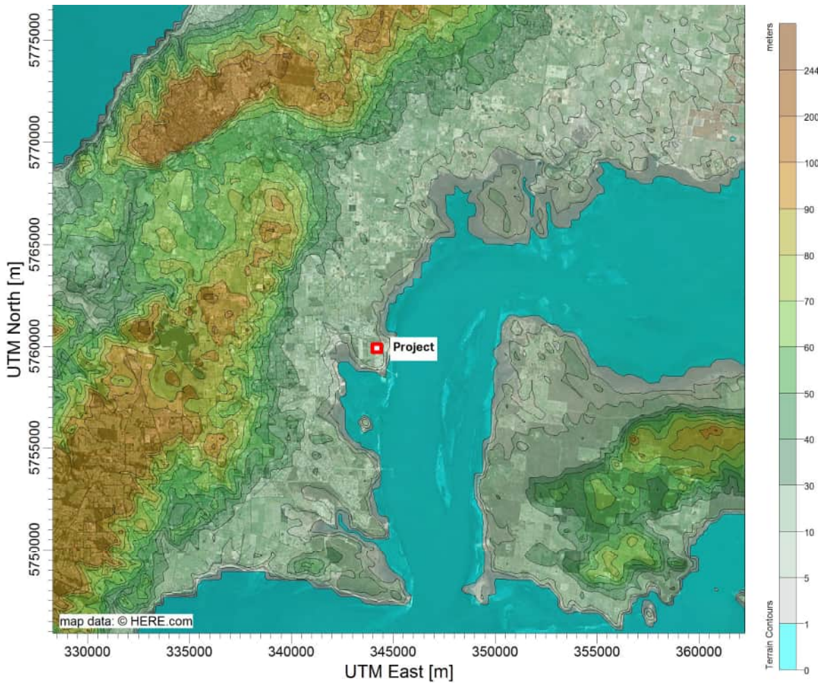
Figure 2 Terrain elevations of model grid
