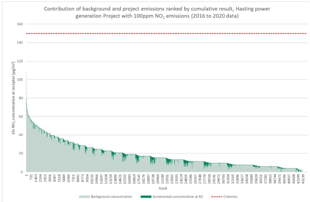
Figure 34 Ranked cumulative NO 2 concentrations at Receptor 2, Hasting power generation Project (with 100ppm NO 2 emissions), 2016 to 2020
