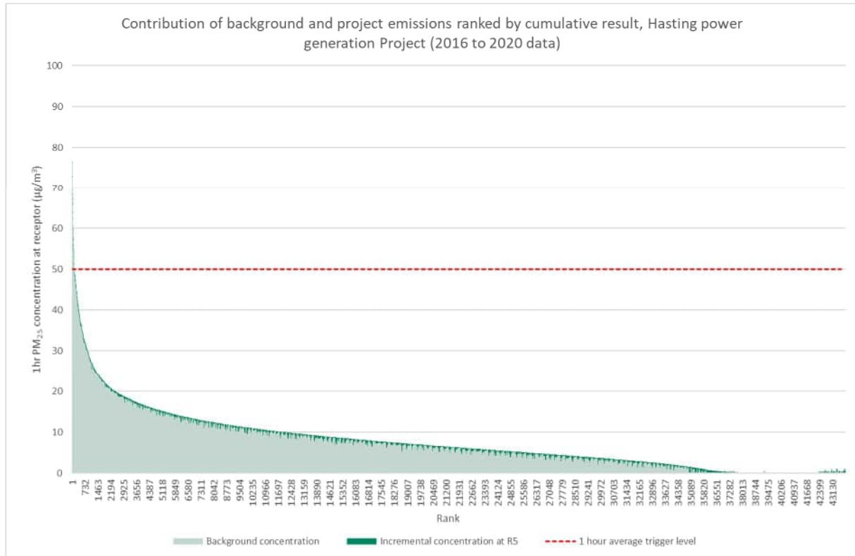
Figure 43 Ranked cumulative PM 2.5 concentrations at Receptor 5, Hasting power generation Project, 2016 to 2020
