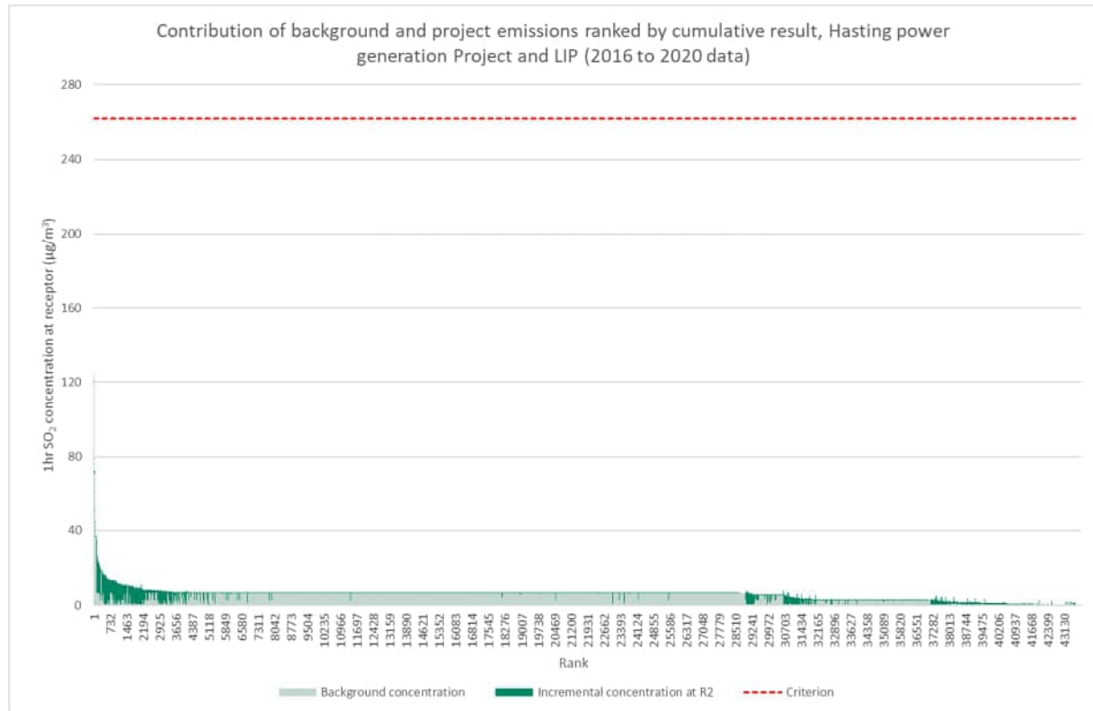
Figure 38 Ranked cumulative SO 2 concentrations at Receptor 2, Hasting power generation Project and LIP, 2016 to 2020
