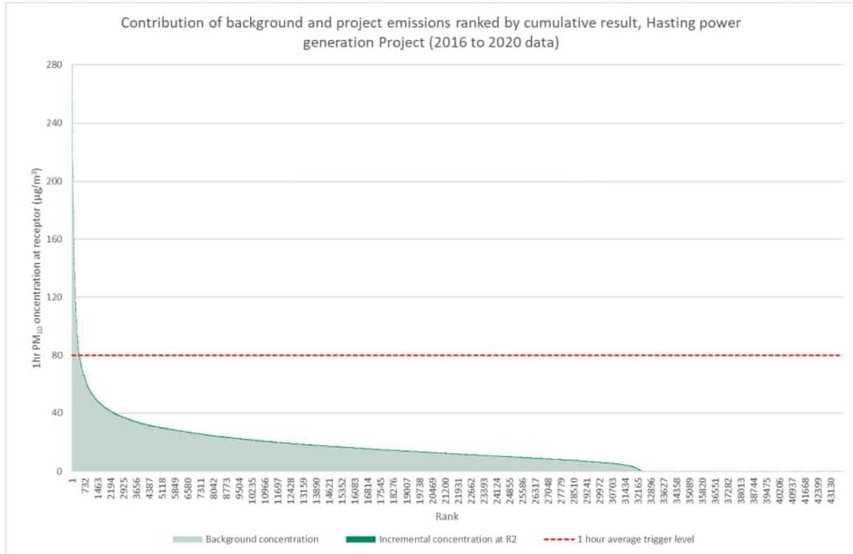
Figure 40 Ranked cumulative PM 10 concentrations at Receptor 2, Hasting power generation Project, 2016 to 2020
