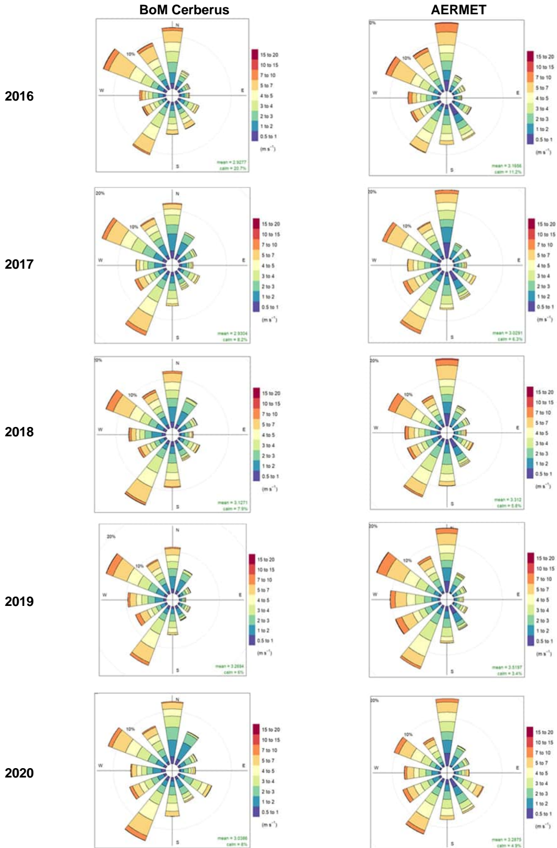
Figure 32 - Annual wind rose comparison, Bom Cerberus vs AERMET
