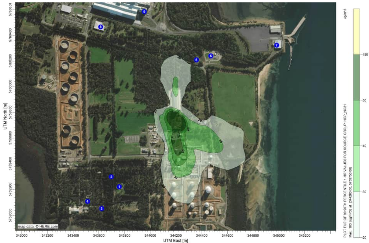
Figure 11 NO 2 results, Hasting power generation Project with 100ppm NO 2 emissions, 1-hr average 99.9 th percentile, no background, 2016 MET (µg/m 3 )
