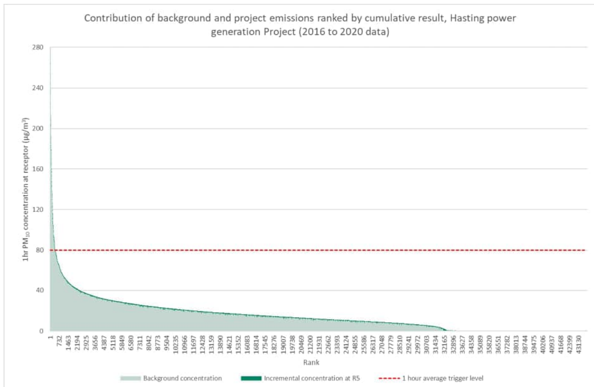
Figure 41 Ranked cumulative PM 10 concentrations at Receptor 5, Hasting power generation Project, 2016 to 2020
