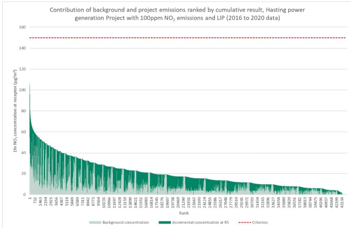
Figure 37 Ranked cumulative NO 2 concentrations at Receptor 5, Hasting power generation Project (with 100ppm NO 2 emissions) and LIP, 2016 to 2020
