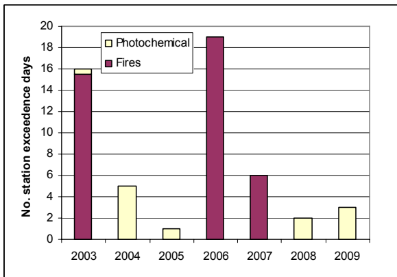
Figure 3: Inferred causes of exceedances of the ozone four-hour standard (Port Phillip region 2003-09)
