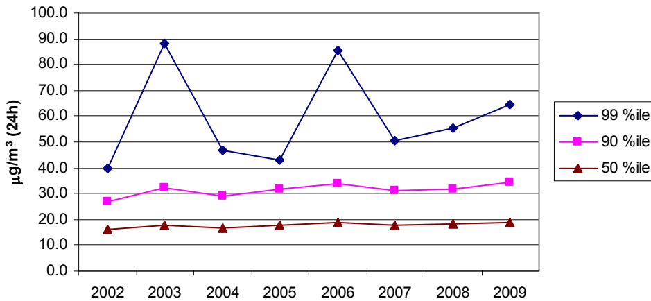
Figure 11: Percentiles of daily PM 10 (average of Port Phillip stations 2002-09)
