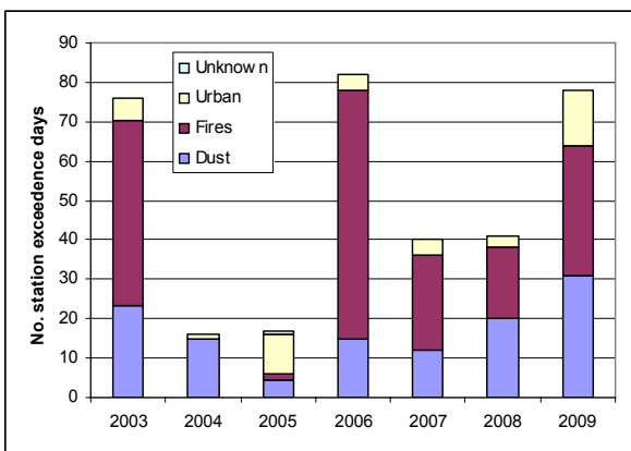
Figure 4: Inferred causes of exceedances of the PM_{10} standard (Port Phillip region 2003-09)
