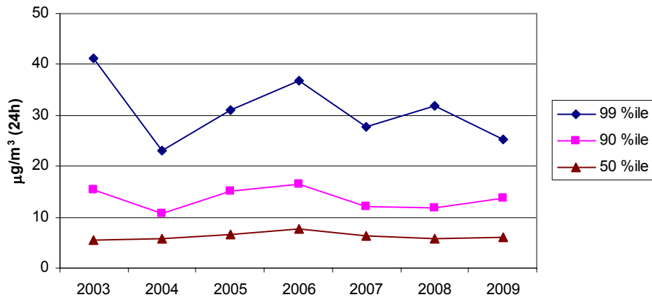
Figure 12: Percentiles of daily PM 2.5 (average of Port Phillip stations 2003-09)
