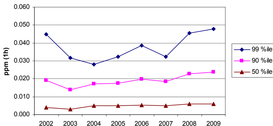
Figure 10: Percentiles of daily maximum one-hour sulfur dioxide (Altona North 2002-09)
