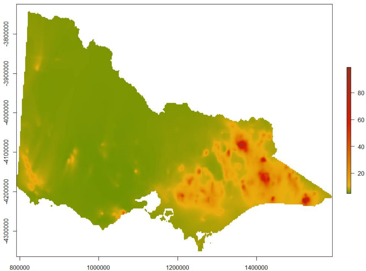
Figure 3: PM 2.5 Population weighted concentration ( \mu\text{g}/\text{m}^3 )
