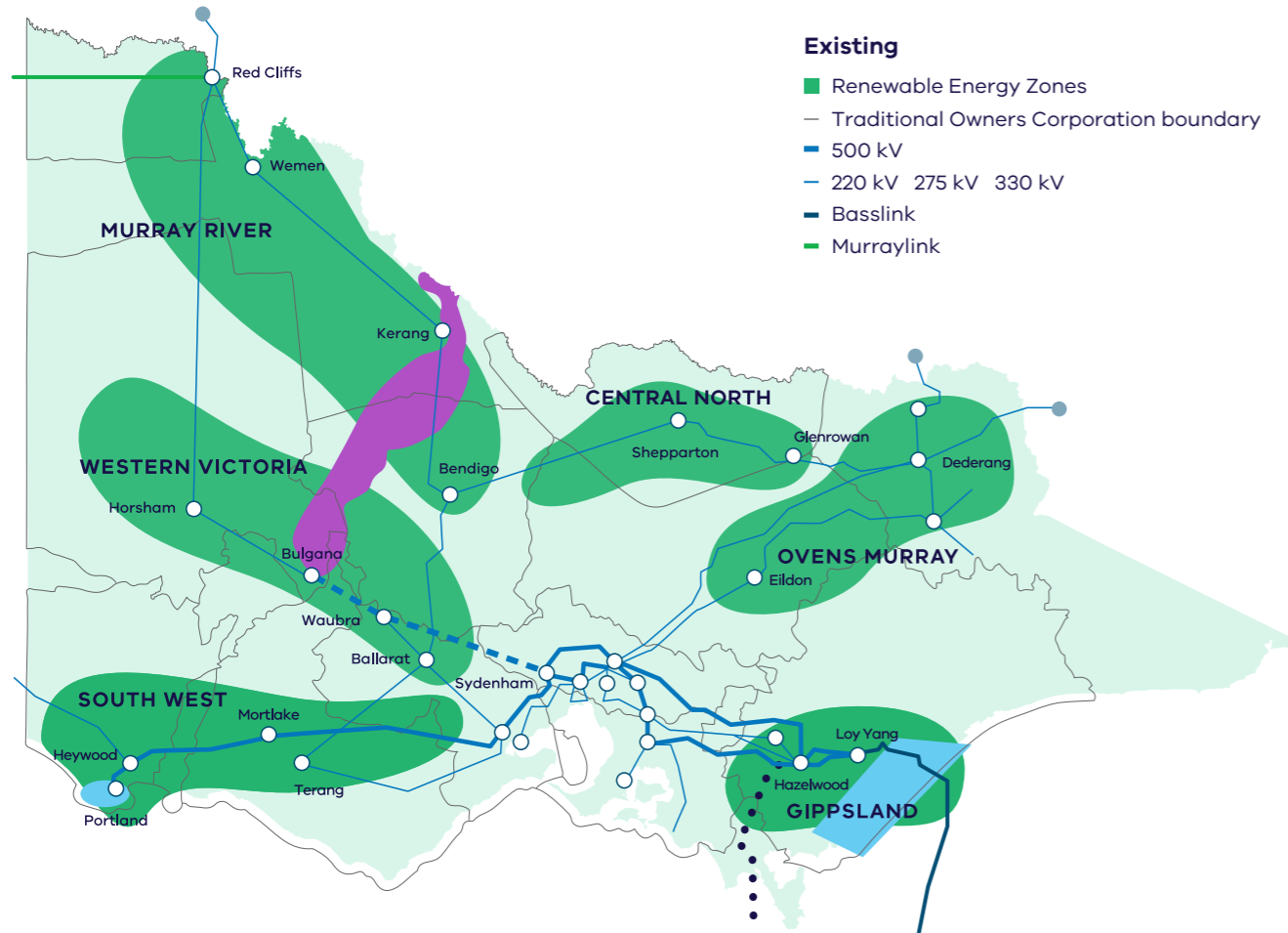
Figure 32 Victoria's Renewable Energy Zones
