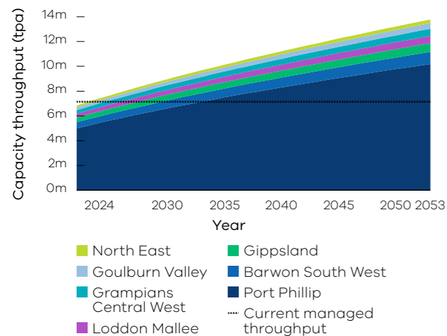
Figure 25 – Aggregates, masonry, and soils reprocessed in Victoria – projected demand and capacity
